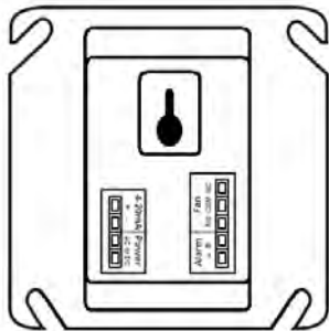
CM-6 rear view with Modular Connectors
